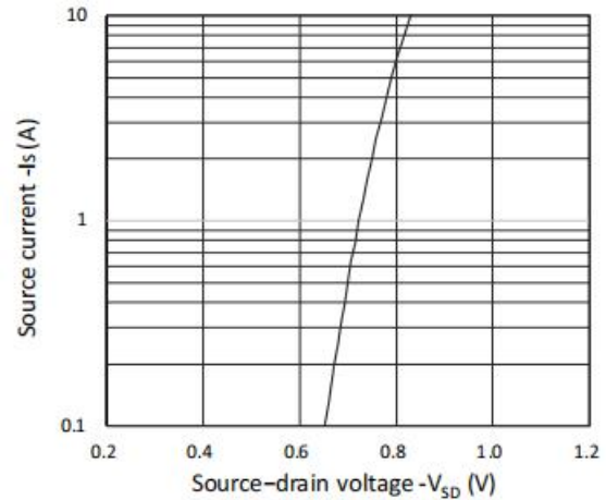
Figure 8: Diode Characteristics
