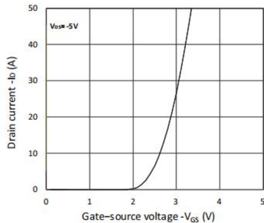
Figure 10: Transfer Characteristics
