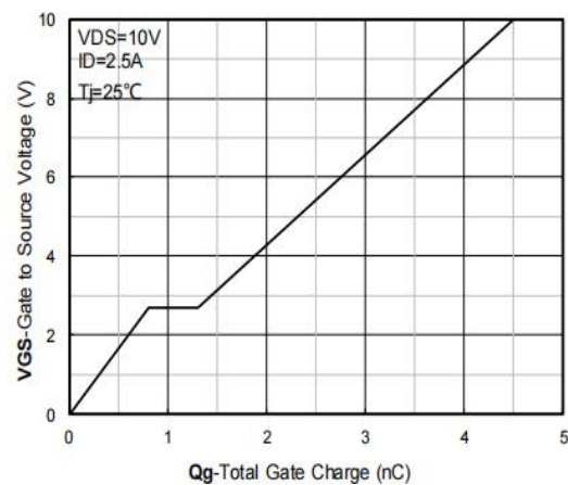
Figure 6: Gate-Charge Characteristics
