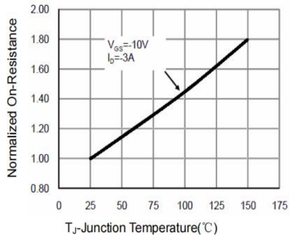
Figure 4: On-Resistance vs.
