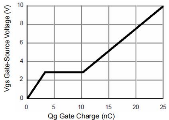
Figure 6: Gate-Charge Characteristics
