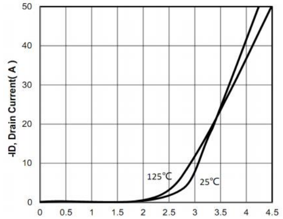
- V_{GS} Gate-Source Voltage (V) Figure 2: Transfer Characteristics
