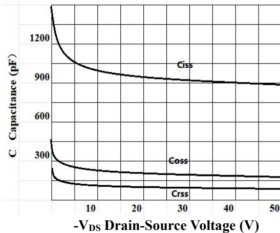
- V_{DS} Drain-Source Voltage (V) Figure 5: Capacitance Characteristics
