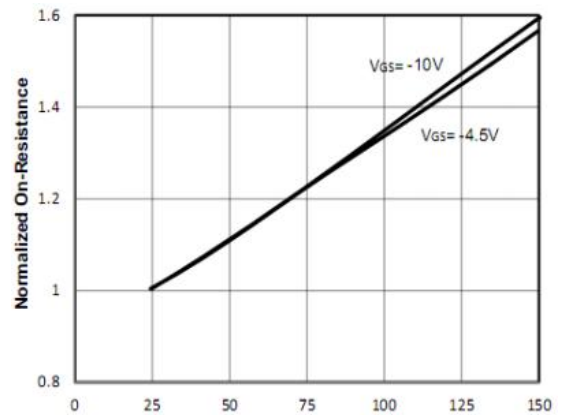
T_J Junction Temperature ( ^{\circ}C ) Figure 4: On-Resistance vs. Temperature
