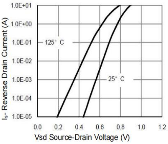
Figure 7: Diode Characteristics
