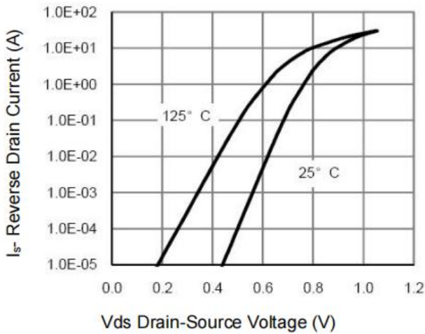
Figure 7: Diode Characteristics
