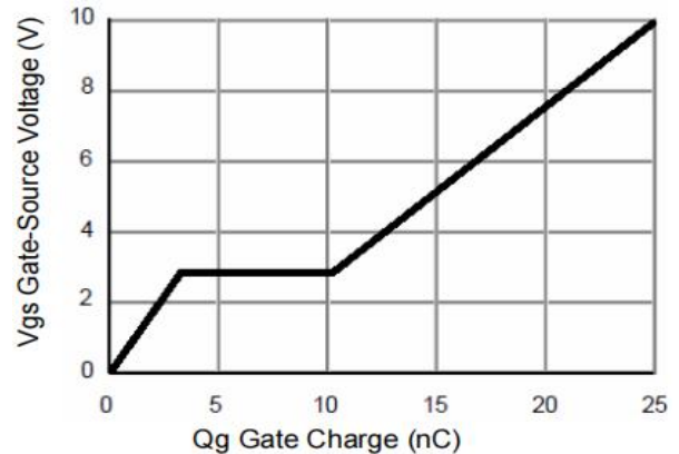
Figure 6: Gate-Charge Characteristics
