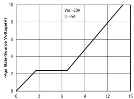
Q g Gate Charge (nC)
