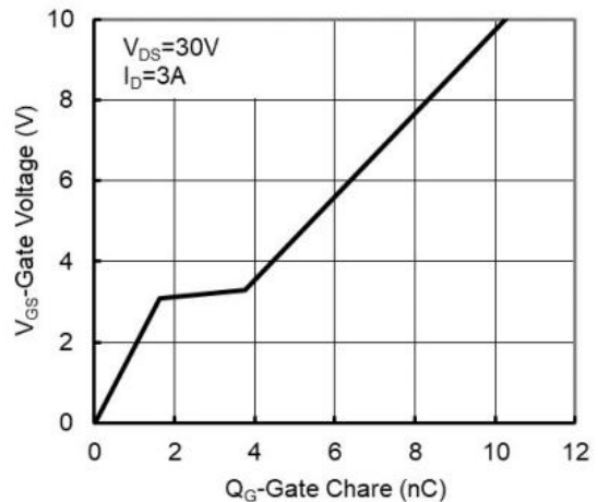
Figure 6: Gate-Charge Characteristics
