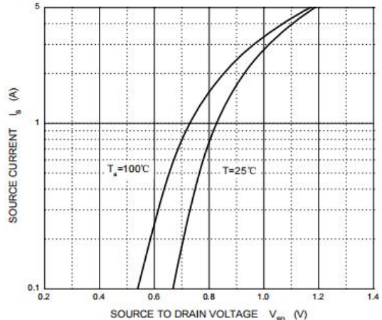
Figure 6: Diode Characteristics
