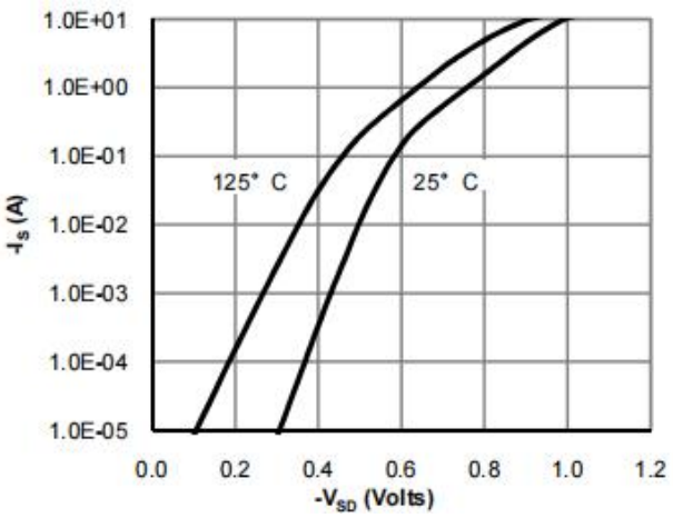
Figure 7: Diode Characteristics
