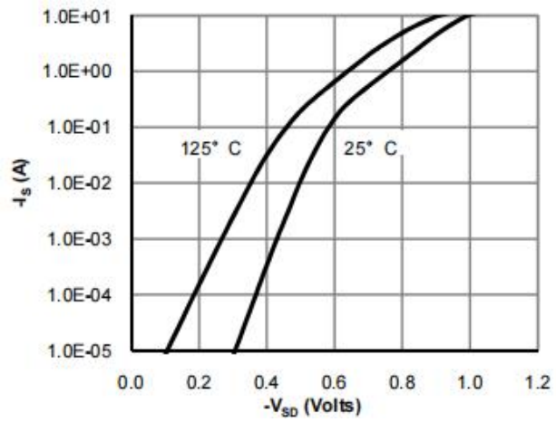
Figure 7: Diode Characteristics
