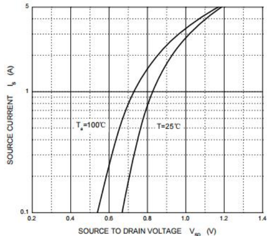
Figure 6: Diode Characteristics
