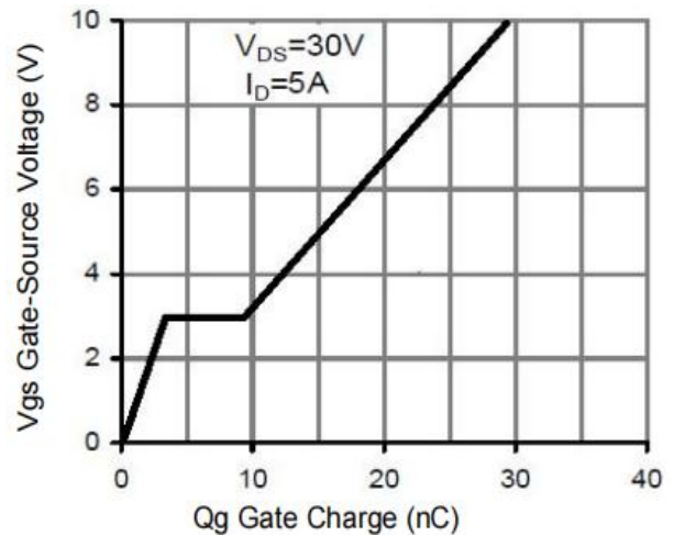
Figure 6: Gate-Charge Characteristics
