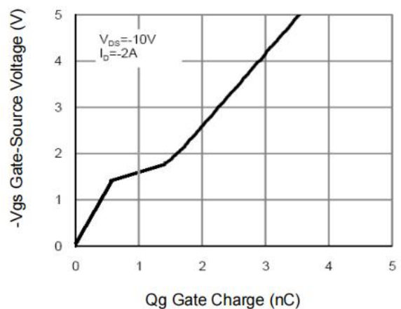
Figure 6: Gate-Charge Characteristics
