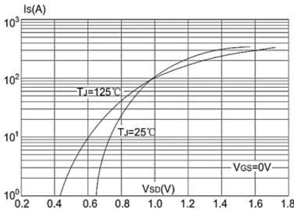
Figure 9: Diode Characteristics
