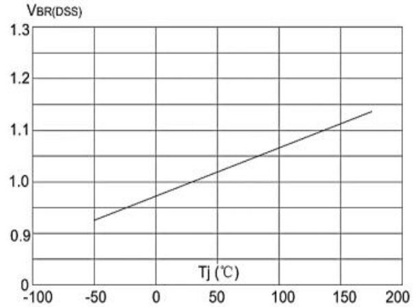
Figure 8: Breakdown Voltage vs. T_j
