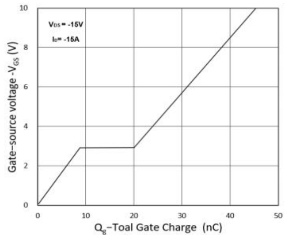
Figure 6: Gate-Charge Characteristics
