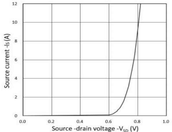
Figure 2: Diode Characteristics
