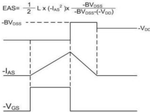
Figure 9: Unclamped Inductive Switching Waveform
