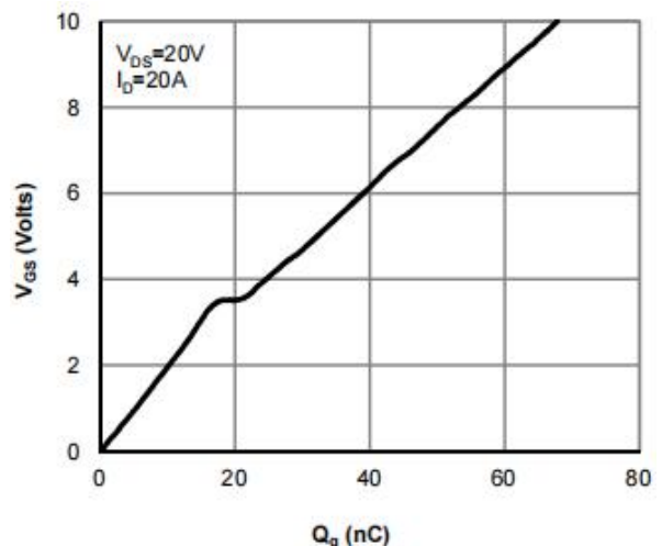
Figure 6: Gate-Charge Characteristics
