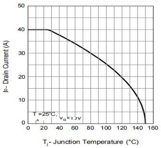
Figure 9: Drain Current Characteristics
