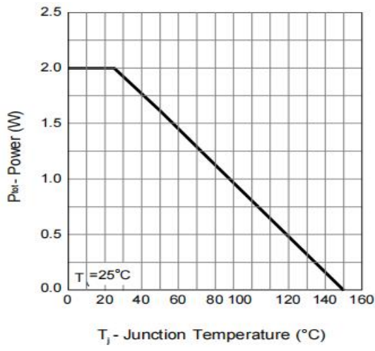
Figure 8: Power Rating Curve
