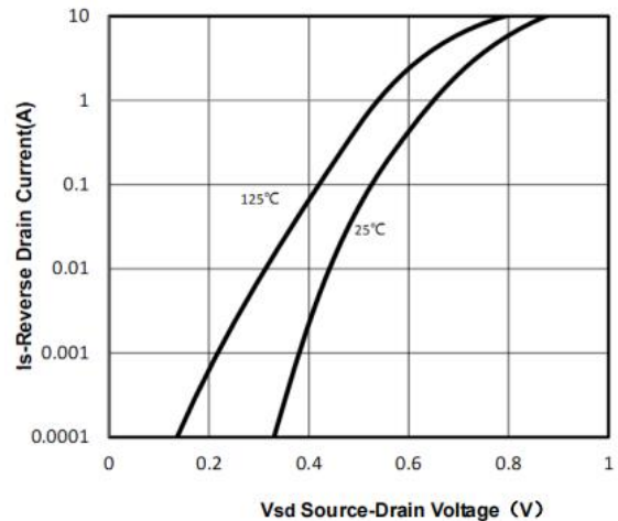
Figure 4: Diode Characteristics
